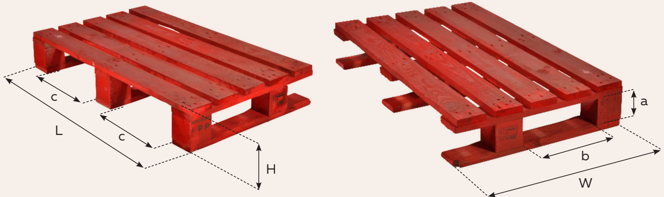
DP610 - Pallet nominal dimensions & tolerance (mm)
